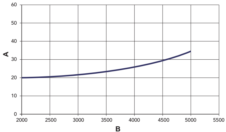
fig. 22 - Pressure loss
