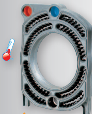
LOW TEMPERATURE CIRCUIT with minimum CH return temperature 35°C
