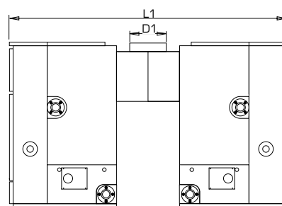
Opposed installation of two boilers with same output
